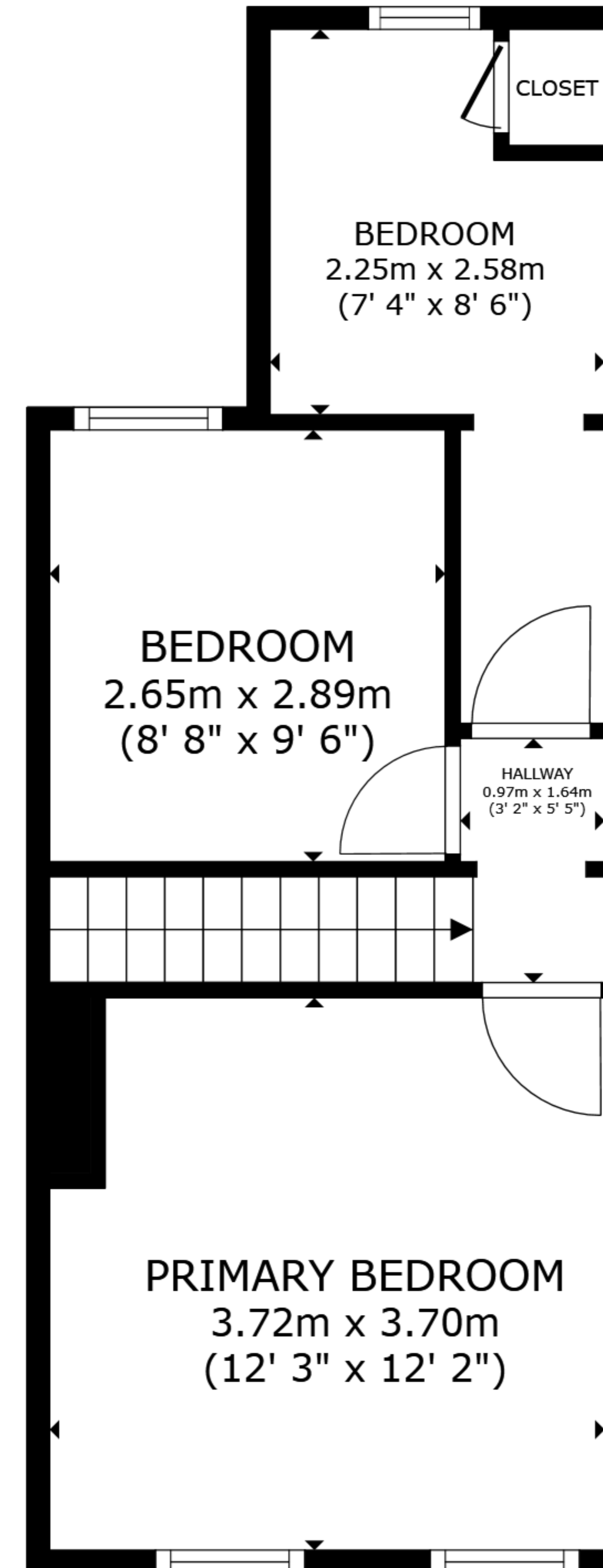
FLOOR 2
